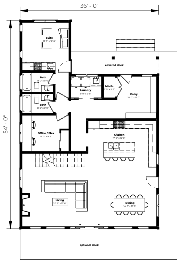
Main Floor Plan 1625 sqft
