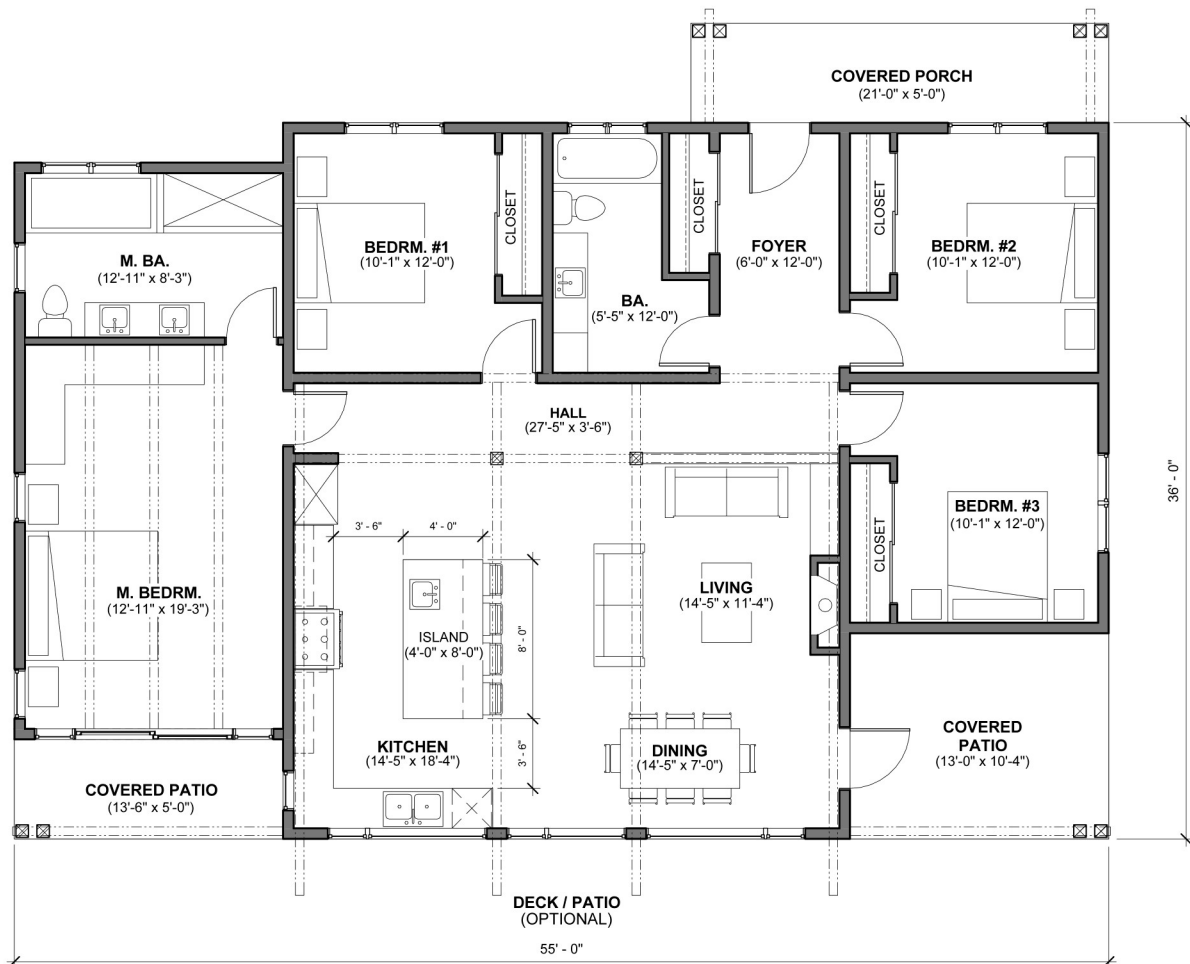
Main Floor 1751 SF
