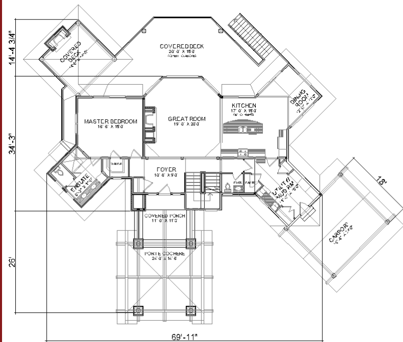
MAIN FLOOR
