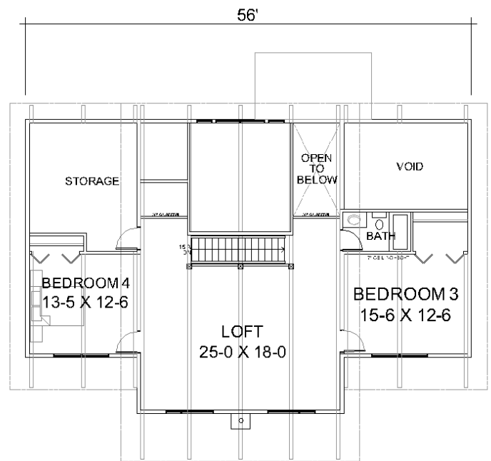
UPPER FLOOR
