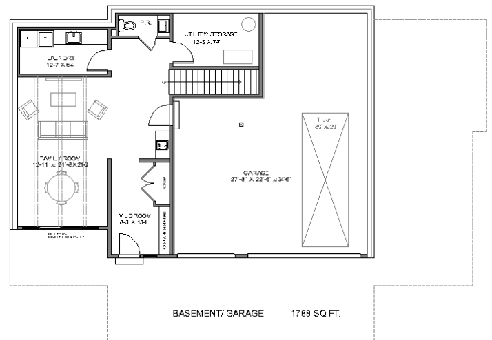
BASEMENT OPTION
