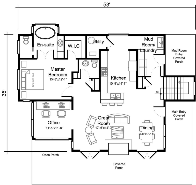
MAIN FLOOR
