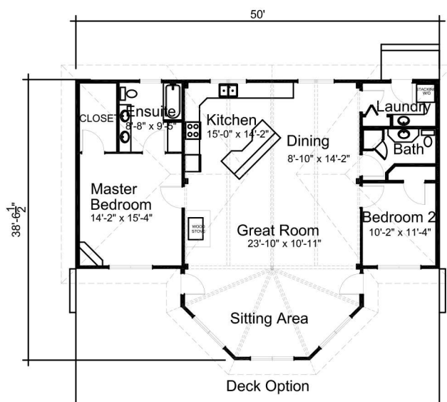
MAIN FLOOR
