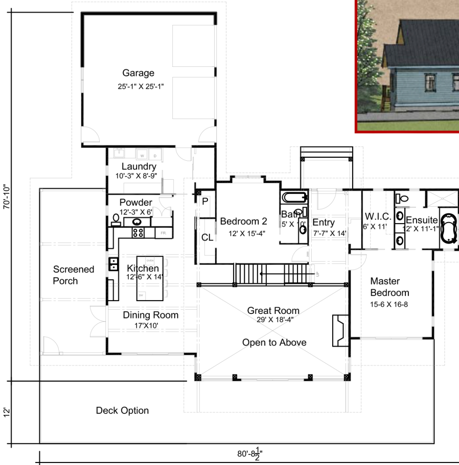
MAIN FLOOR
