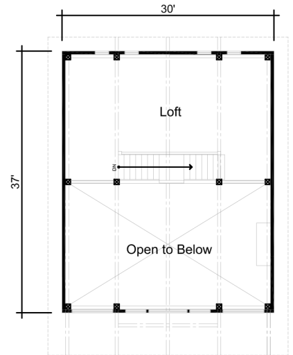
LOFT FLOOR
